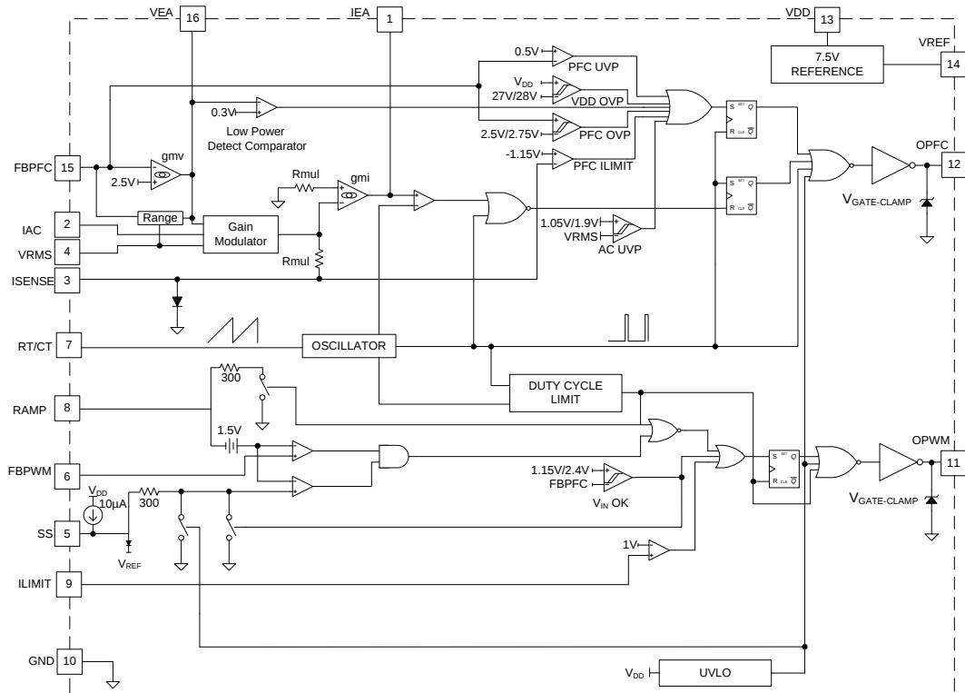
Figure 4. FAN4801S/I02S Function Block Diagram
