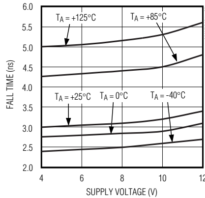
FALL TIME vs. SUPPLY VOLTAGE
