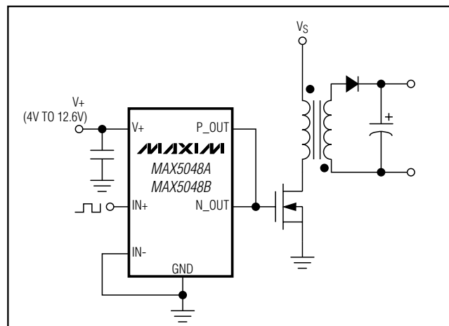
Figure 3. Noninverting Application
