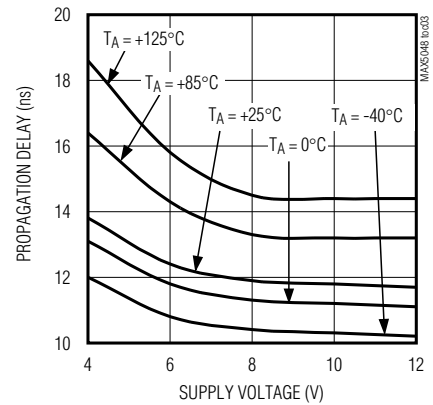
PROPAGATION DELAY TIME, LOW-TO-HIGH vs. SUPPLY VOLTAGE
