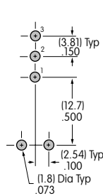
Single Pole
