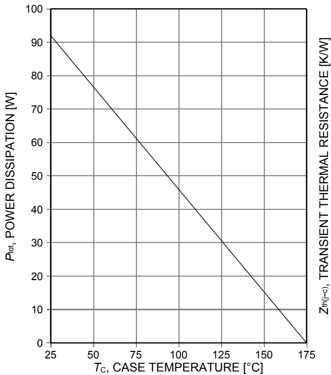
Figure 1. Power dissipation per diode as a function of case temperature ( T_{vj} \leq 175^\circ\text{C} )
