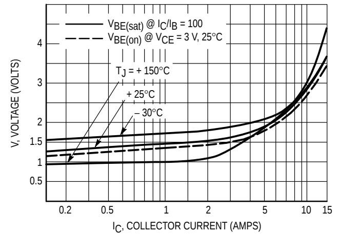
Figure 5. Base-Emitter Voltage
