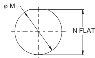
Jam-Nut Panel Cut Out
