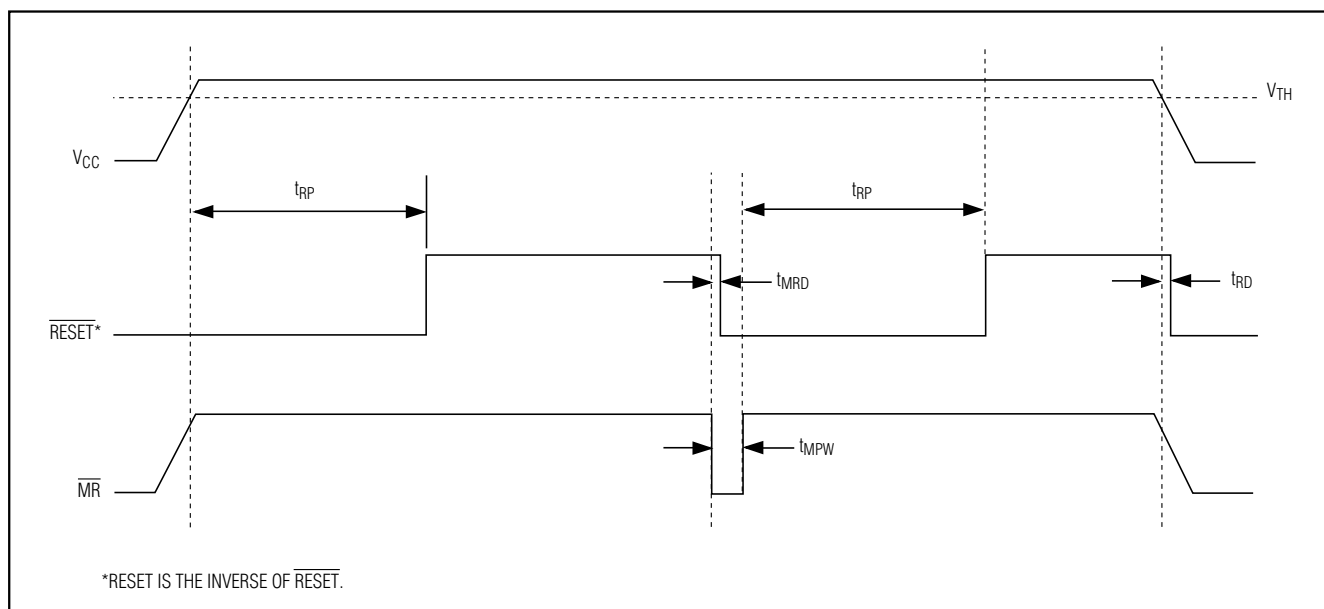
Figure 2. \overline{RESET} Timing Relationship
