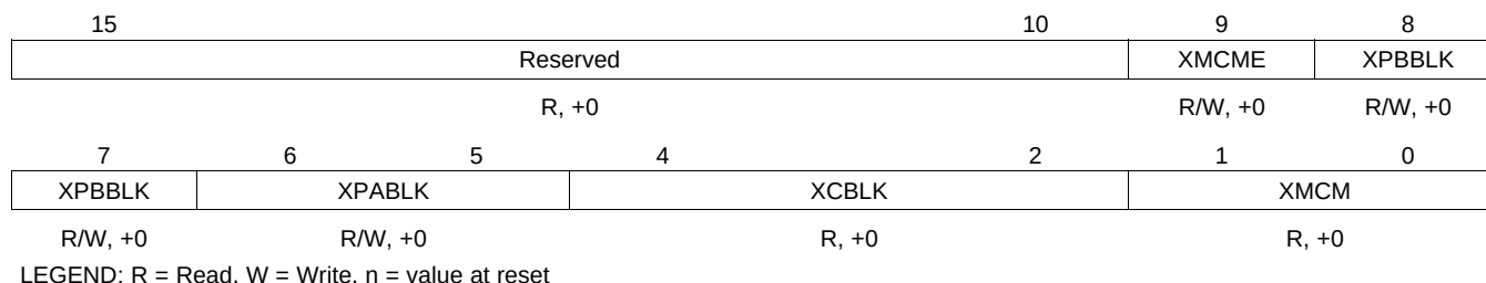
Figure 3-11. Multichannel Control Register 2x (MCR2x)
