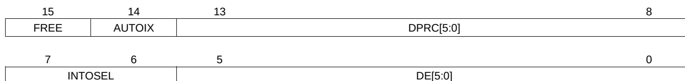
Figure 3-22. DMPREC Register
