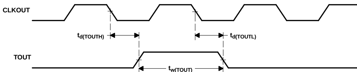
Figure 5-20. TOUT Timing
