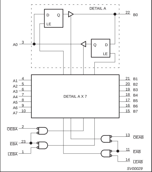
LOGIC DIAGRAM
