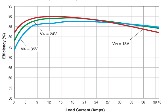
UCQ-2.5/40-D24 Efficiency vs Line Voltage and Load Current @25° C
