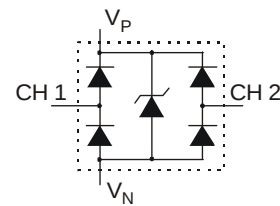
Device Schematic
