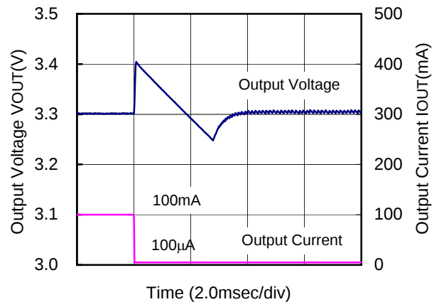
XC9104D092MR(PWM/PFM,180kHz,3.3V)
