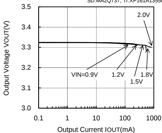
XC9104D093MR (PWM/PFM,300kHz,3.3V)
