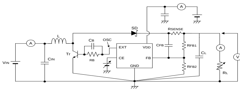
CIRCUIT ②
