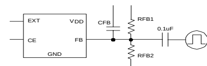
CIRCUIT ⑥
