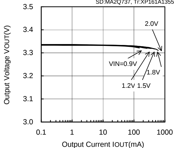
XC9103D095MR (PWM,500kHz,3.3V)
