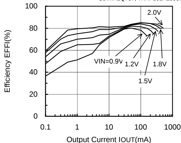
XC9104D092MR (PWM/PFM,180kHz,3.3V)
