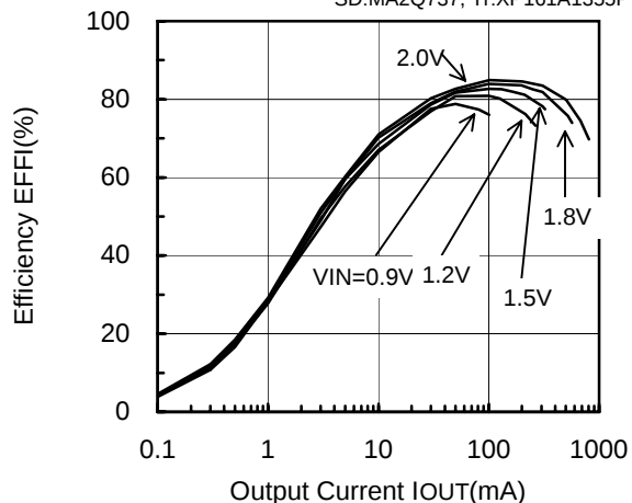
XC9103D093MR (PWM,300kHz,3.3V)
