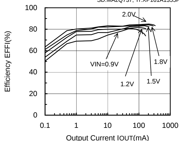
XC9104D091MR (PWM/PFM,100kHz,3.3V)
