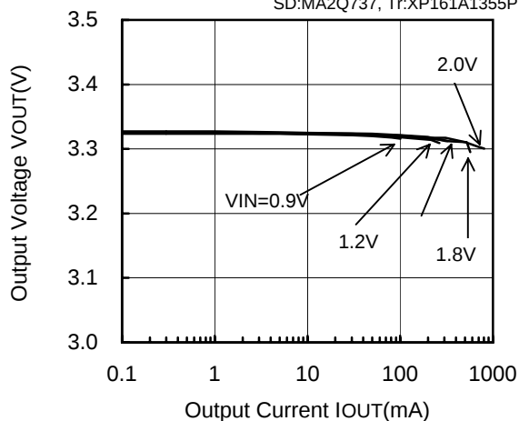
XC9103D093MR (PWM,300kHz,3.3V)
