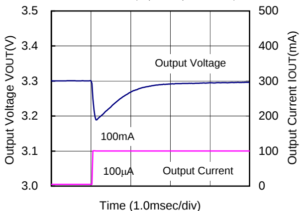
XC9103D093MR(PWM,300kHz,3.3V)
