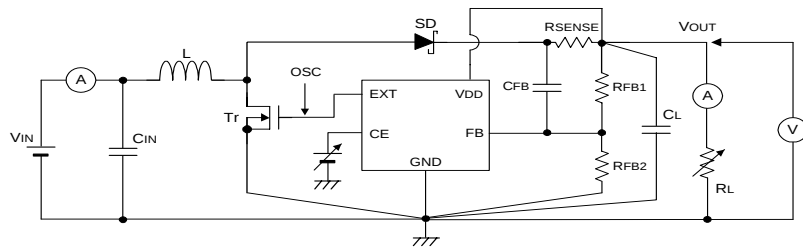
CIRCUIT ①
