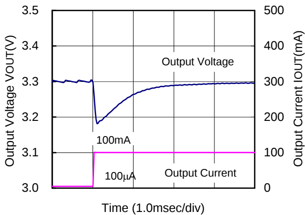
XC9104D092MR(PWM/PFM,180kHz,3.3V)
