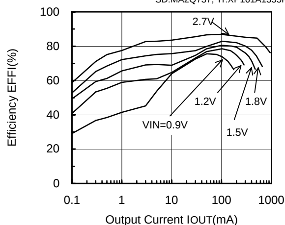
XC9104D093MR (PWM/PFM,300kHz,3.3V)
