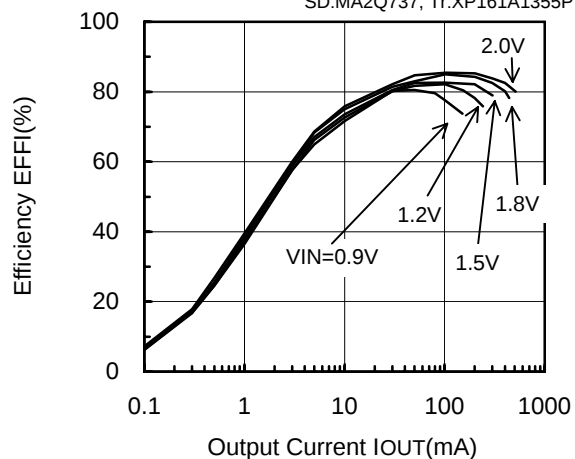
XC9103D092MR (PWM,180kHz,3.3V)
