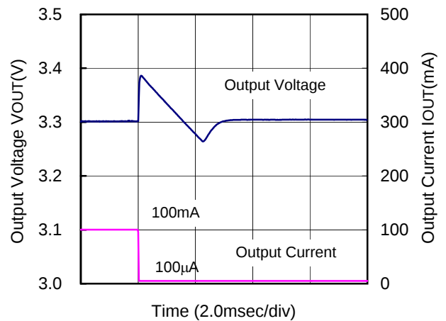
XC9103D092MR(PWM,180kHz,3.3V)
