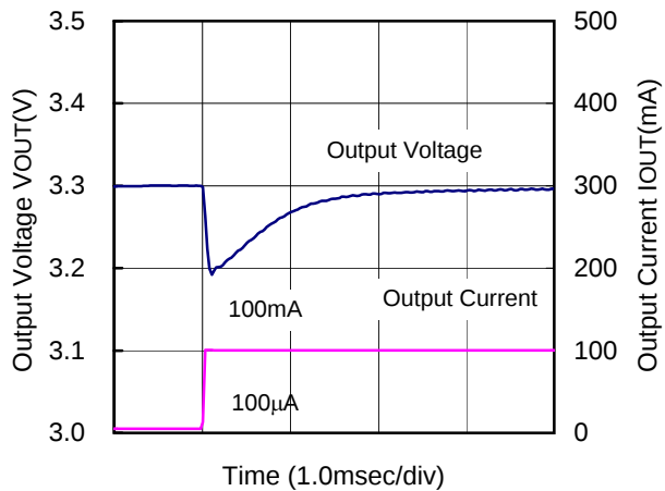
XC9103D092MR(PWM,180kHz,3.3V)
