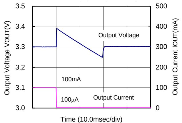
XC9103D093MR(PWM,300kHz,3.3V)
