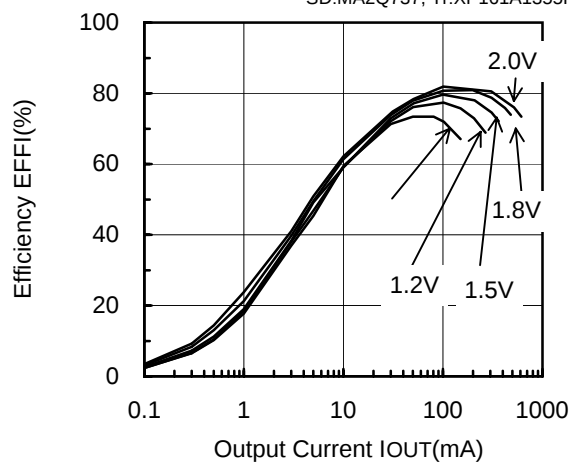
XC9103D095MR (PWM,500kHz,3.3V)
