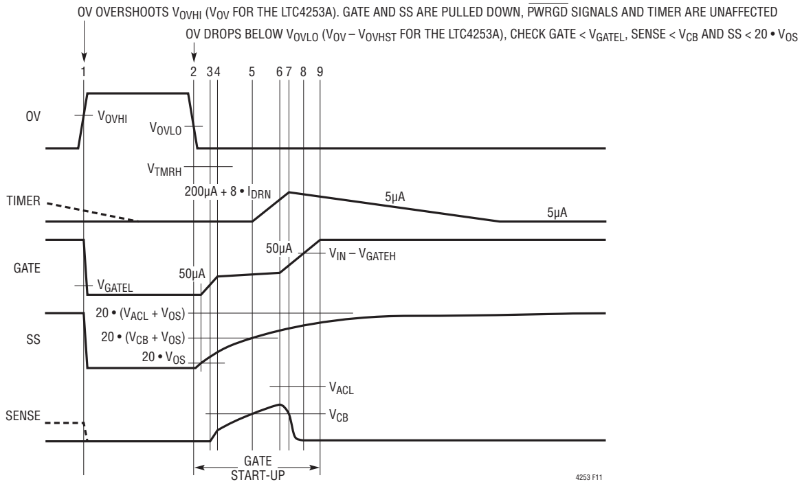
Figure 11. Overtiming Timing (All Waveforms Are Referenced to V_{EE} )
