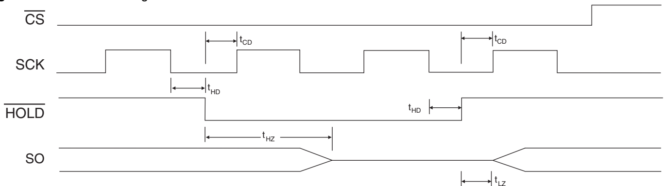
Figure 4-8. HOLD Timing
