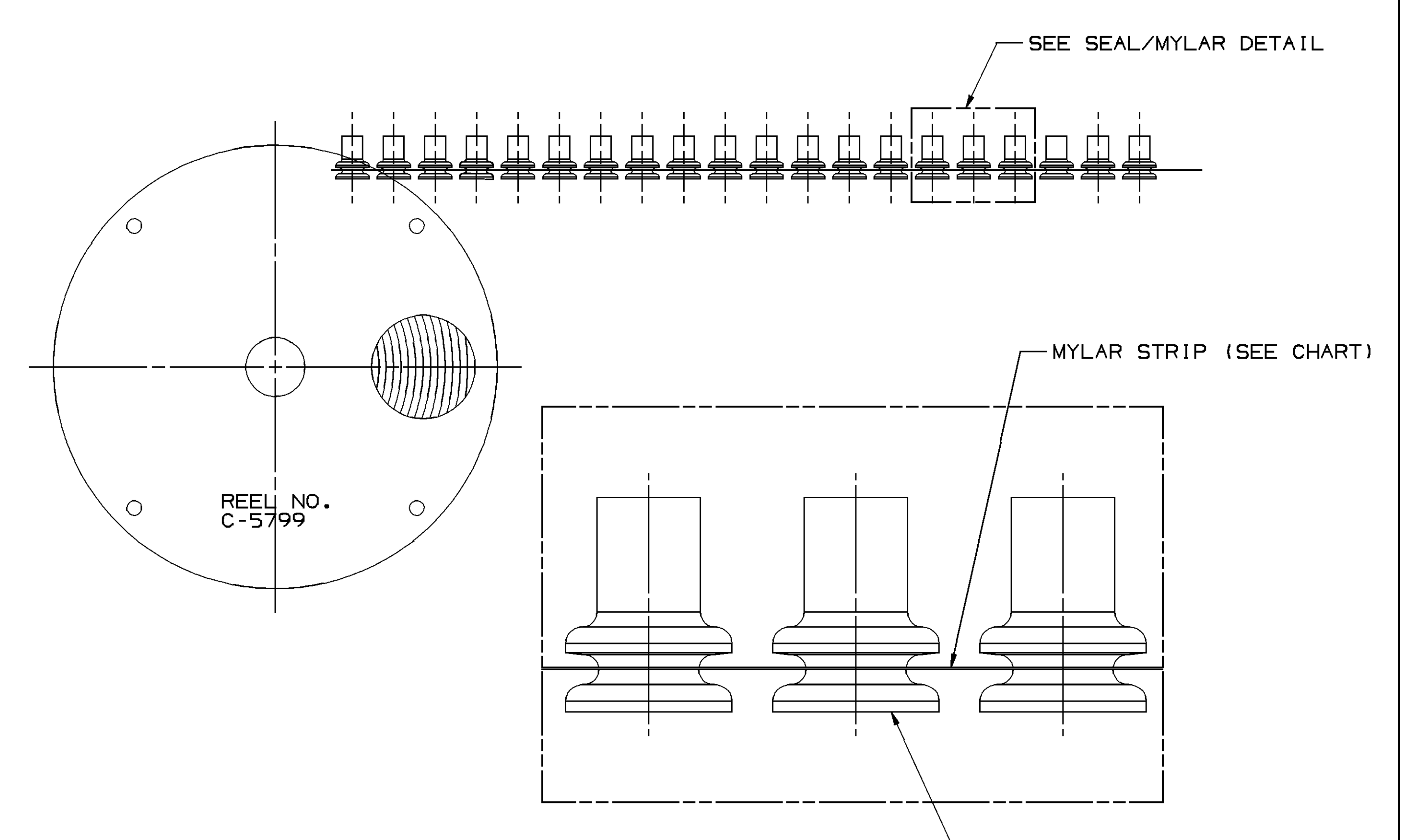
SEAL/MYLAR ASSEMBLY DETAIL NO SCALE TYPE 102 SAME AS TYPE 101 EXCEPT AS SHOWN
