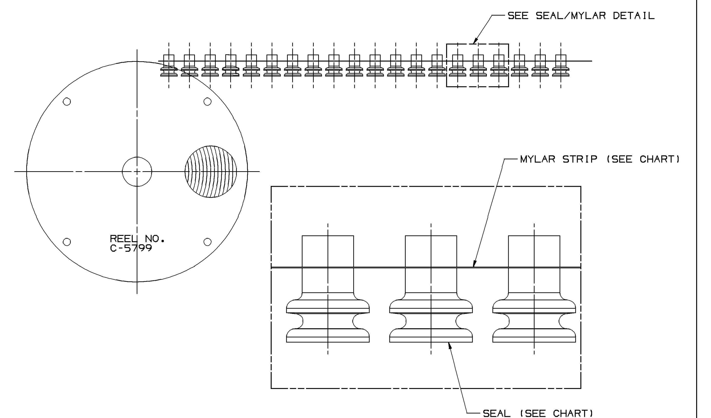
SEAL/MYLAR ASSEMBLY DETAIL NO SCALE TYPE 101
