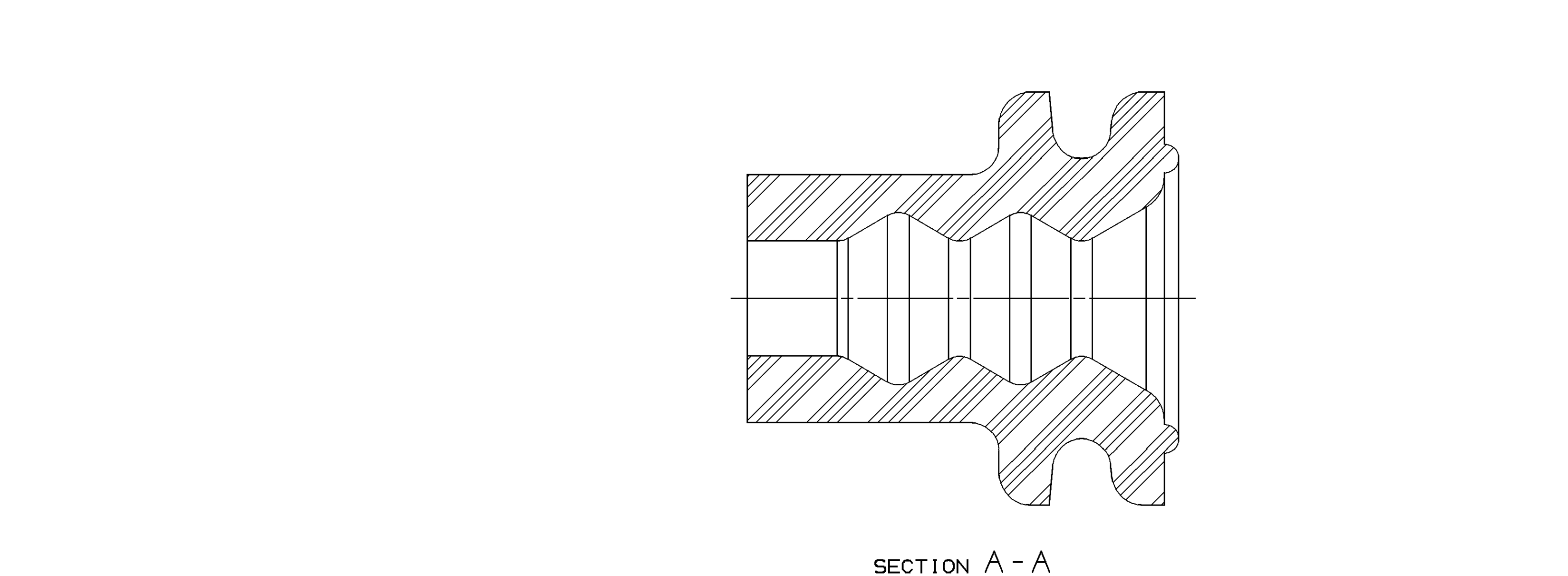
GT 150 3.5 CL (3.2 X 4.0 OVAL INTERNAL CAVITY DIAMETER)
