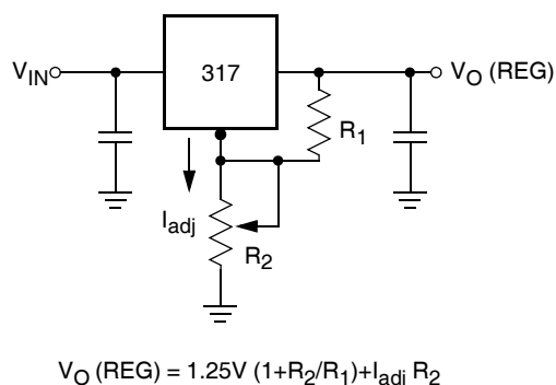
Voltage Regulator
