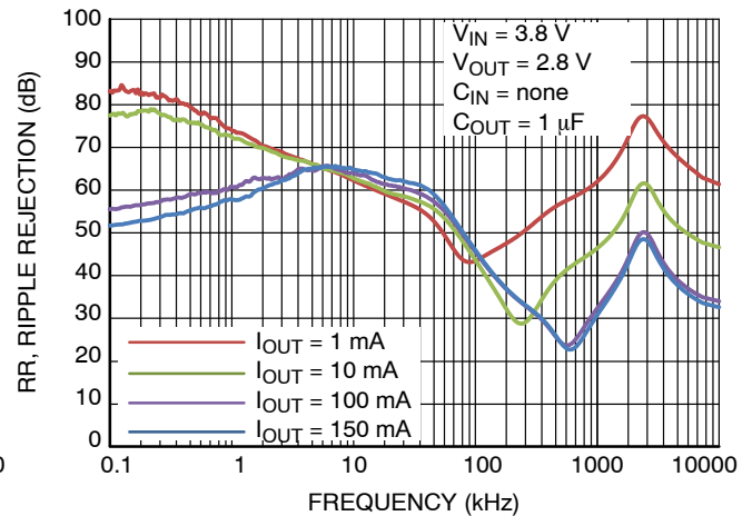
Figure 26. Power Supply Rejection Ratio, V_{OUT} = 2.8\text{ V} , C_{OUT} = 1\text{ }\mu\text{F}
