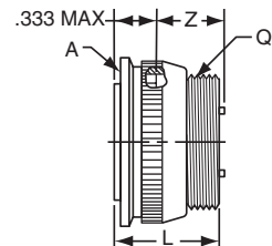
"P" Potting Boot
