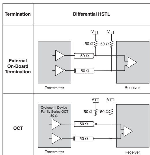
Figure 6-8. Cyclone III Device Family Differential HSTL I/O Standard Termination
