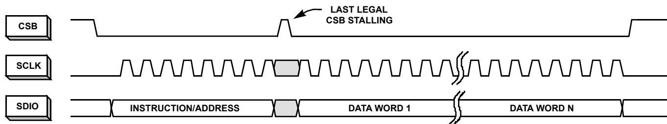
FIGURE 44. N-BYTE TRANSFER
