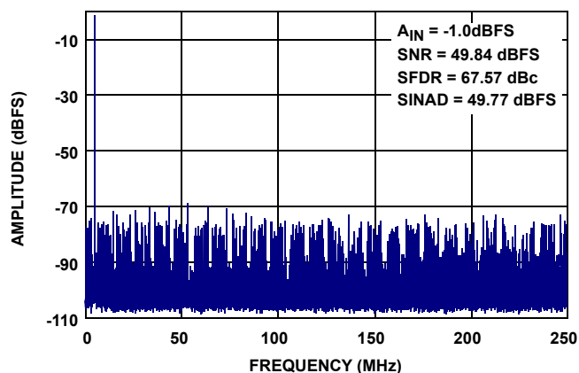
FIGURE 18. SINGLE-TONE SPECTRUM @ 495MHz
