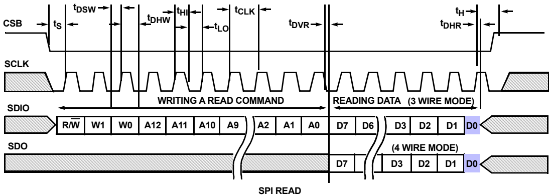
FIGURE 42. SPI READ
