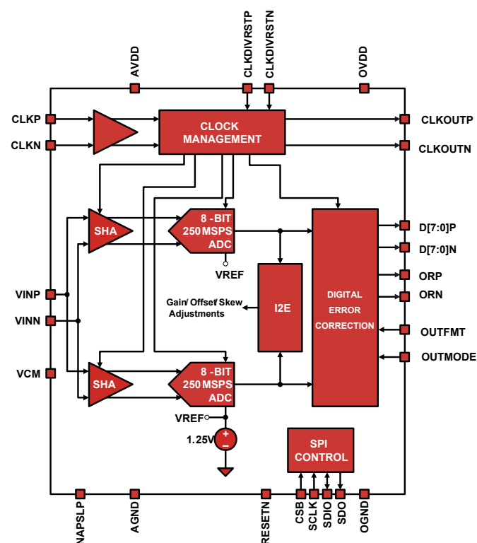
FIGURE 1. BLOCK DIAGRAM
