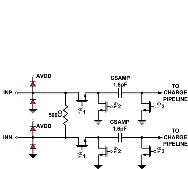
FIGURE 47. ANALOG INPUTS
