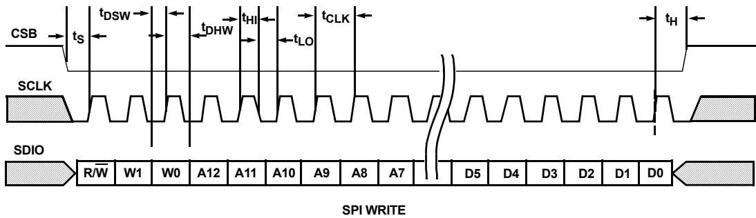
SPI WRITE
