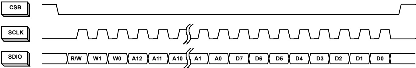
FIGURE 39. MSB-FIRST ADDRESSING
