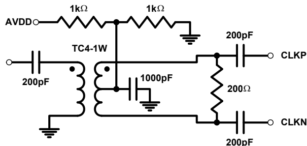
FIGURE 34. RECOMMENDED CLOCK DRIVE
