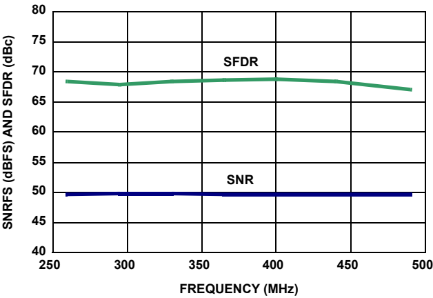
FIGURE 23. INPUT FREQUENCY SWEEP WITH I2E FROZEN, I2E PREVIOUSLY CALIBRATED @ 330MHz
