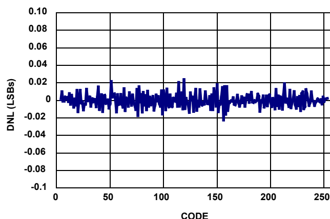
FIGURE 12. DIFFERENTIAL NONLINEARITY
