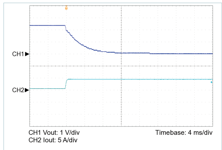
Figure 8 — 10% to 100% load transient response, V_{IN} = 24\text{ V} , nominal trim, C_{OUT\_EXT} = 200\text{ }\mu\text{F}
