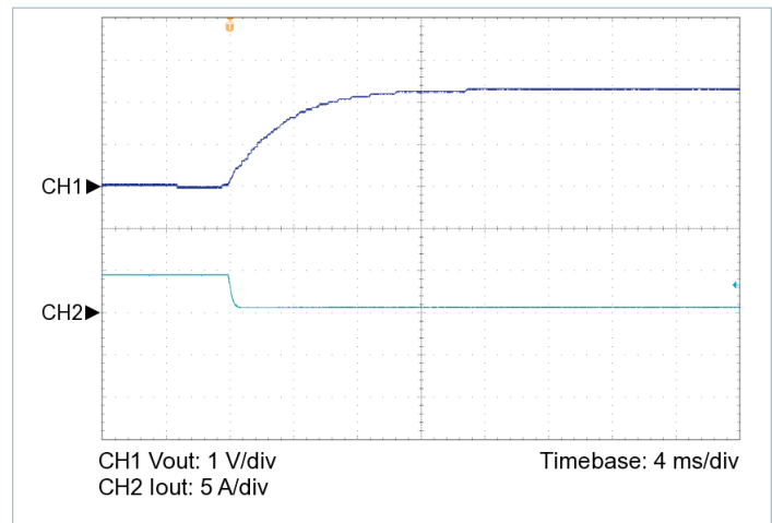
Figure 7 — 100% to 10% load transient response, V_{IN} = 24\text{ V} , nominal trim, C_{OUT\_EXT} = 200\text{ }\mu\text{F}
