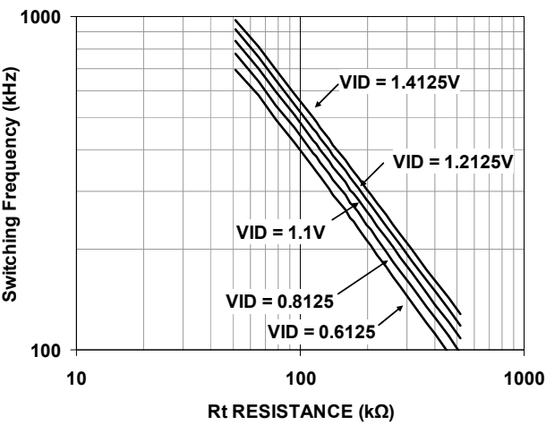
Figure 8. Per Phase Switching Frequency vs. RT Resistance
