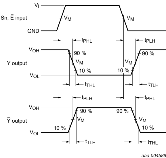
Measurement points are given in Table 8 . V_{OL} and V_{OH} are typical voltage output levels that occur with the output load. Fig 6. Propagation delay input (Sn, \bar{E} ) to output (Y, \bar{Y} ) and output (Y, \bar{Y} ) transitions time
