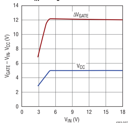
\Delta V_{GATE} and V_{CC} Voltages vs V_{IN} Voltage
