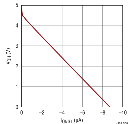
ONST Output High Voltage vs Current
