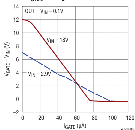
\Delta V_{GATE} Voltage vs Current
