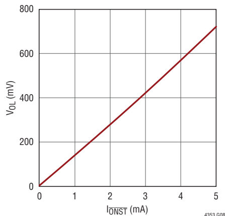
ONST Output Low Voltage vs Current
