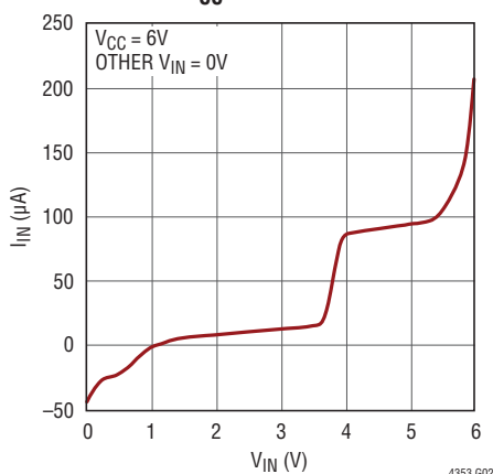
V_{IN} Current vs Voltage with External V_{CC}
