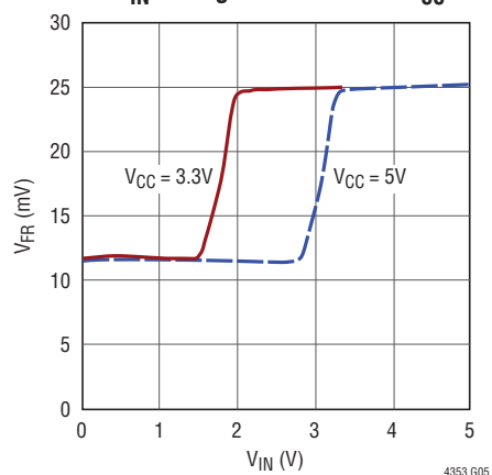
Forward Regulation Voltage vs V_{IN} Voltage with External V_{CC}
