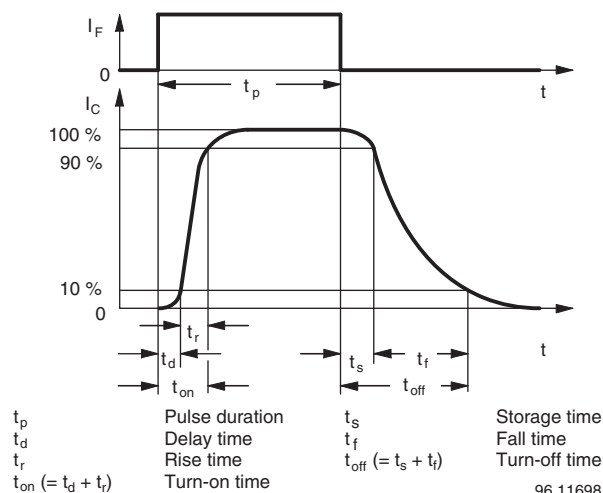
Fig. 5 - Switching Times
