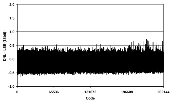
TPC 4. Differential Nonlinearity vs. Code
