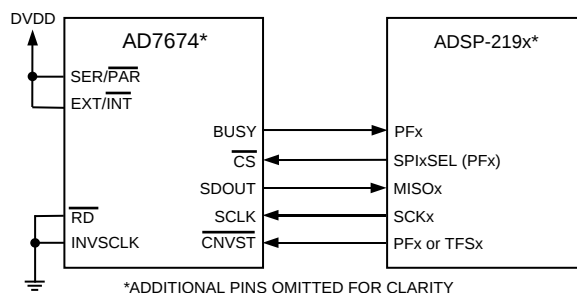
Figure 23. Interfacing the AD7674 to SPI Interface
