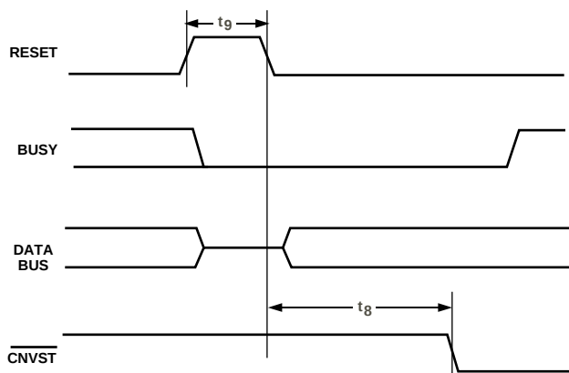
Figure 13. RESET Timing
