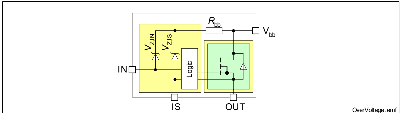
Figure 15 Over-Voltage Protection
