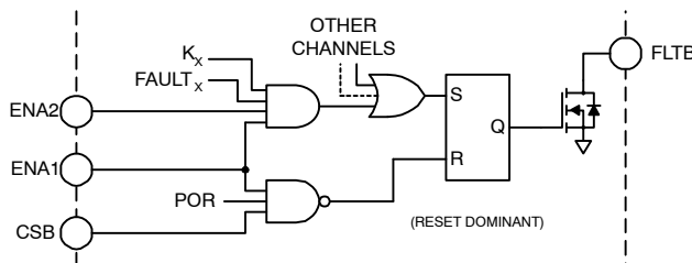
Figure 18. FLT_B Flag Logic
