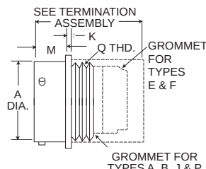
CRIMP KPSE00/MS3120
