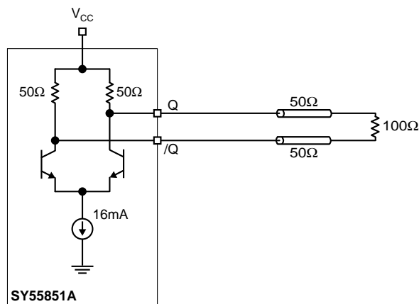
Figure 3b. Differentially Terminated SY55851A ( 50\Omega Load CML Output)
