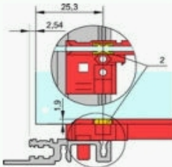
Optionally with ESD clip
