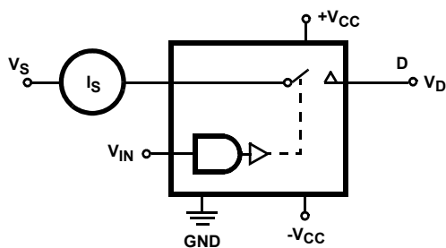
FIGURE 4. I_S (OFF)
