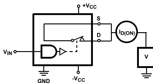
FIGURE 5. I_D (ON)
