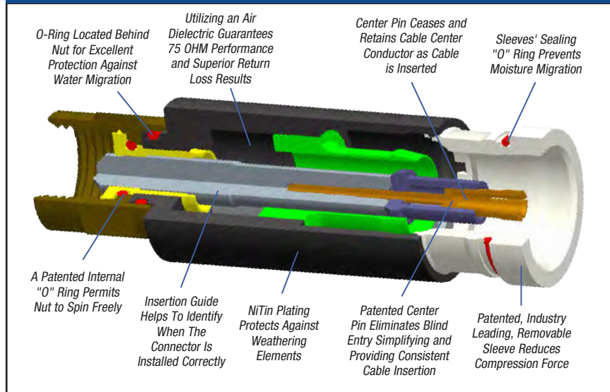
Internal Depiction of a ProSNS™ RG-11 Connector
