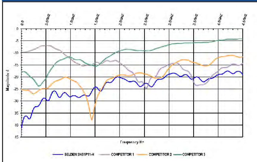
ProSNS™ RG-11 Connector RL Performance
