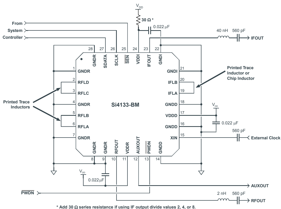
Figure 14. Si4133-BM
