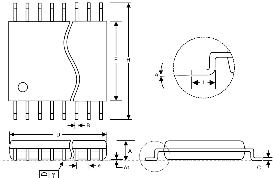
Figure 19. 24-Pin Thin Shrink Small Outline Package (TSSOP)
