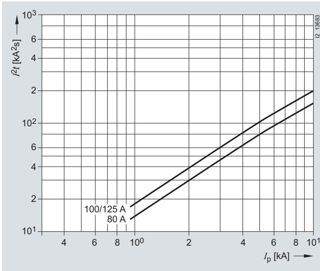
Characteristic C
