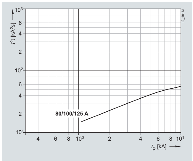
Characteristic C
