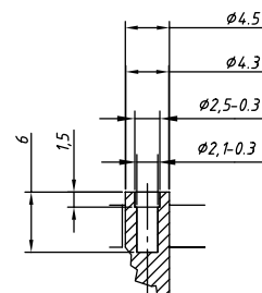
Detail Z
