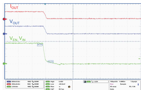
Figure 40. Turn-off time
