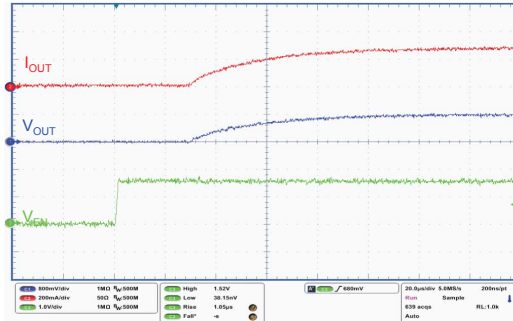
Figure 35. Startup by enable
