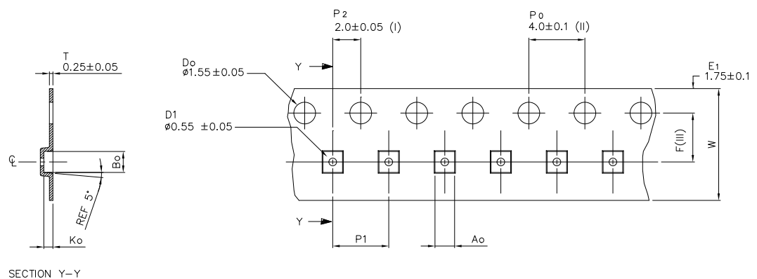
Figure 54. DFN6 tape
