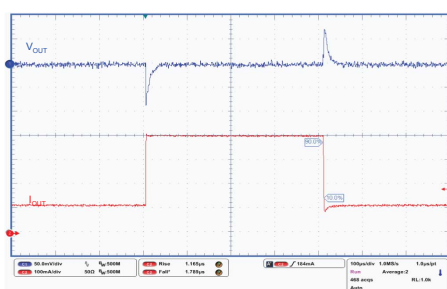
Figure 45. Load transient ( I_{OUT} = 1 to 300 mA, normal mode)
