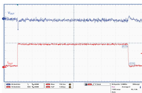
Figure 45. Load transient ( I_{OUT} = 1 to 300 mA, normal mode)
