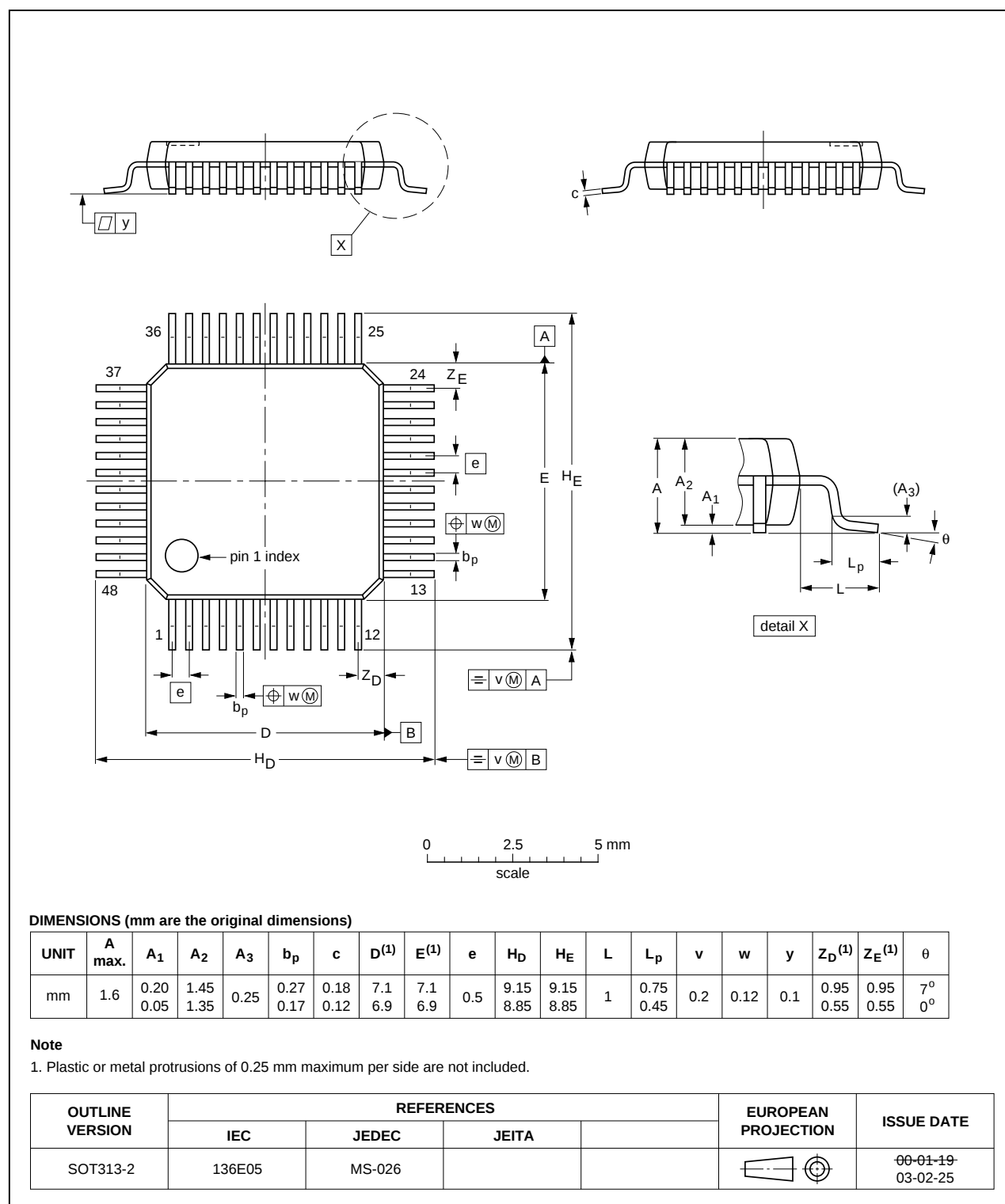
Fig 45. Package outline LQFP48 (SOT313-2)
