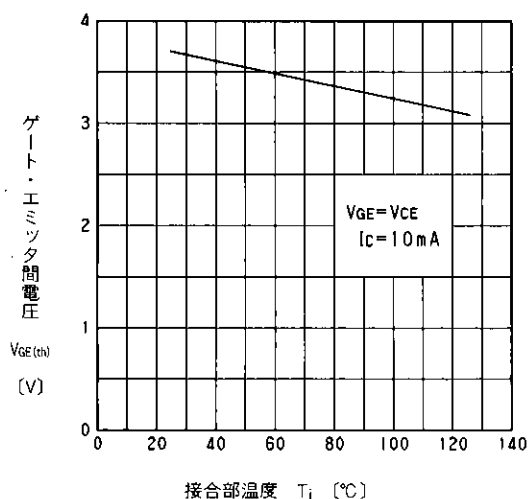
Gate Threshold Voltage vs. Junction Temperature
