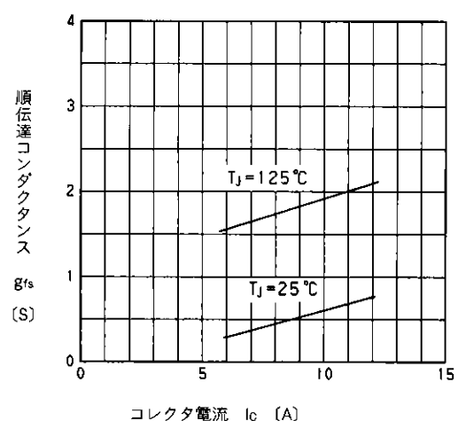
Typical Transconductances
