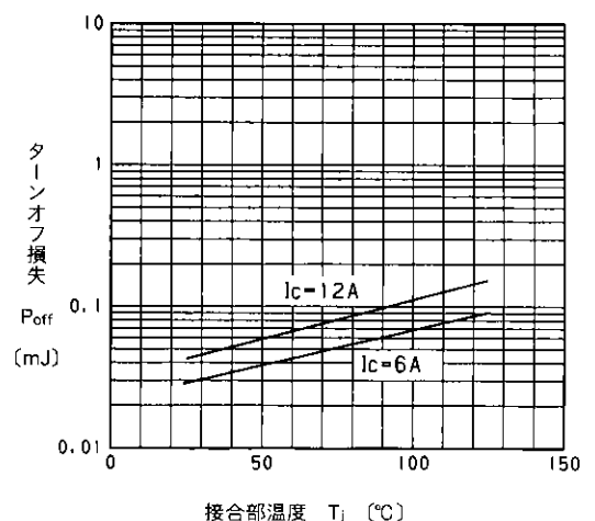
P_{off} - T_J Characteristics
