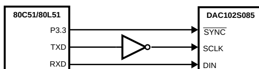
Figure 39. 80C51/80L51 Interface
