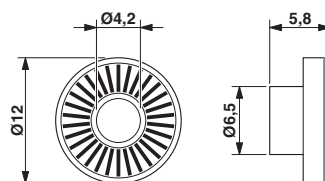
Dimensioned drawing
