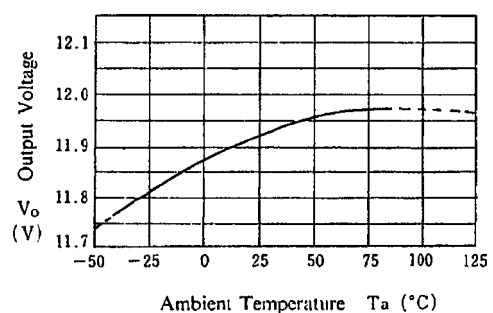
NJM78L12 Output Voltage vs. Temperature
