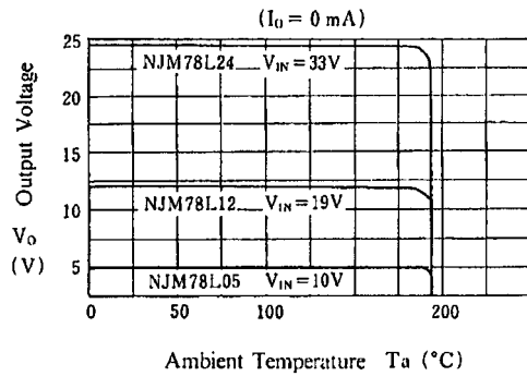
Thermal Shutdown Characteristics
