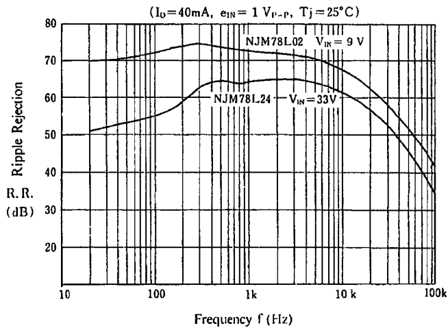
NJM78L02 / L24 Ripple Rejection
