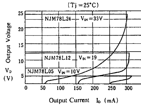
Load Characteristics
