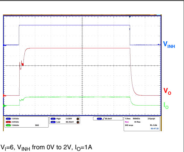
Figure 27. INH transient
