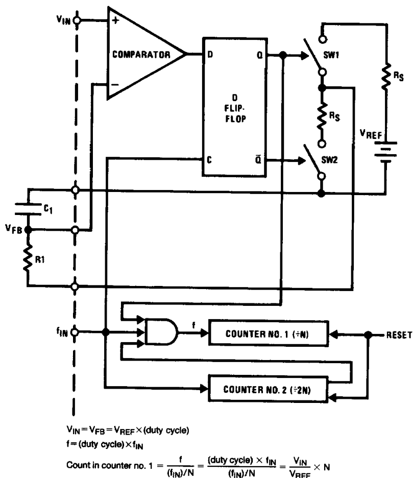
FIGURE 1. Analog Loop Schematic Pulse Modulation A/D Converter
