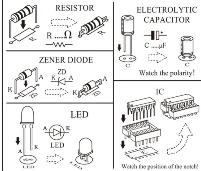
Figure 3 Installing components
