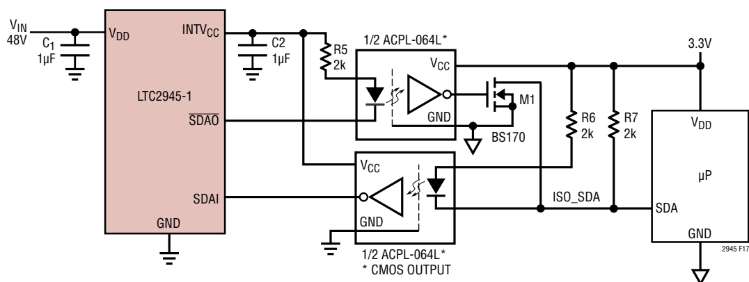
Figure 17. Opto-Isolation of I²C Interface with Low Power, High Speed Opto-couplers (SCL Omitted for Clarity)
