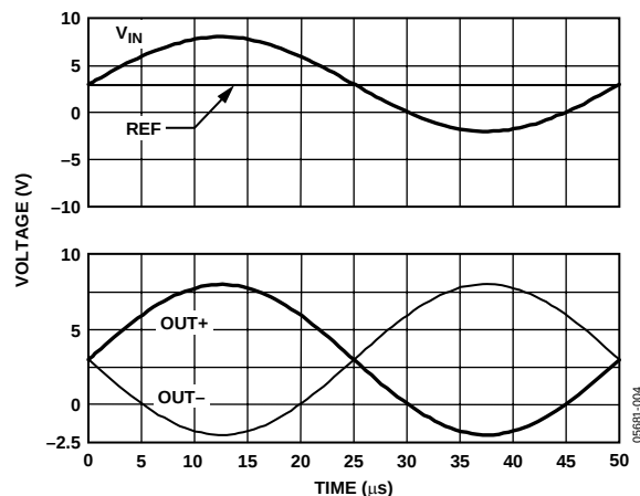
Figure 43. Typical Input/Output Response—Equal Input/Reference
