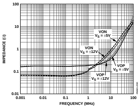
Figure 21. Single-Ended Output Impedance vs. Frequency and Supplies
