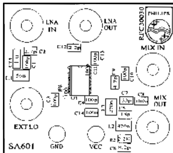
Silk Screen
