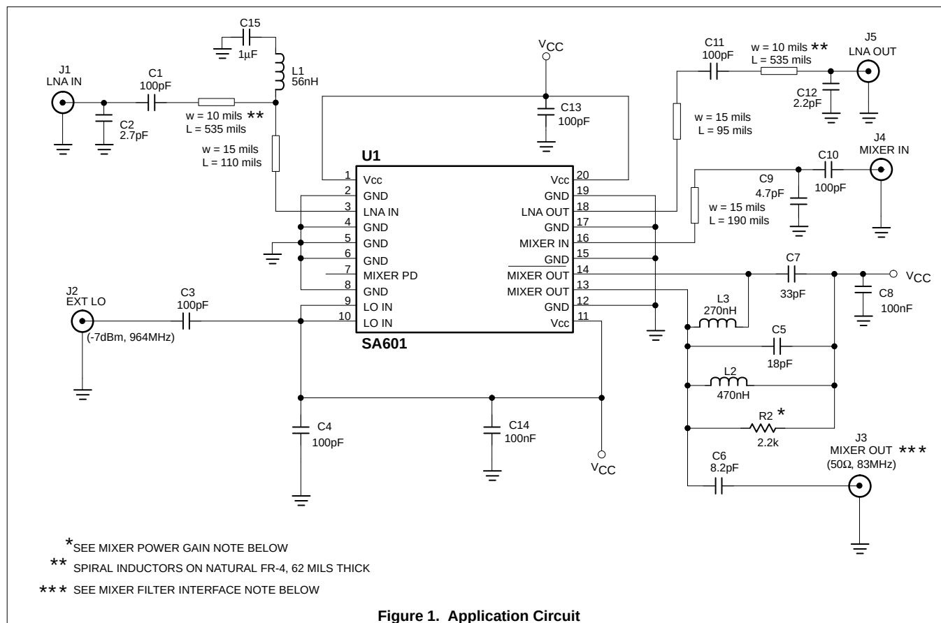
Figure 1. Application Circuit
