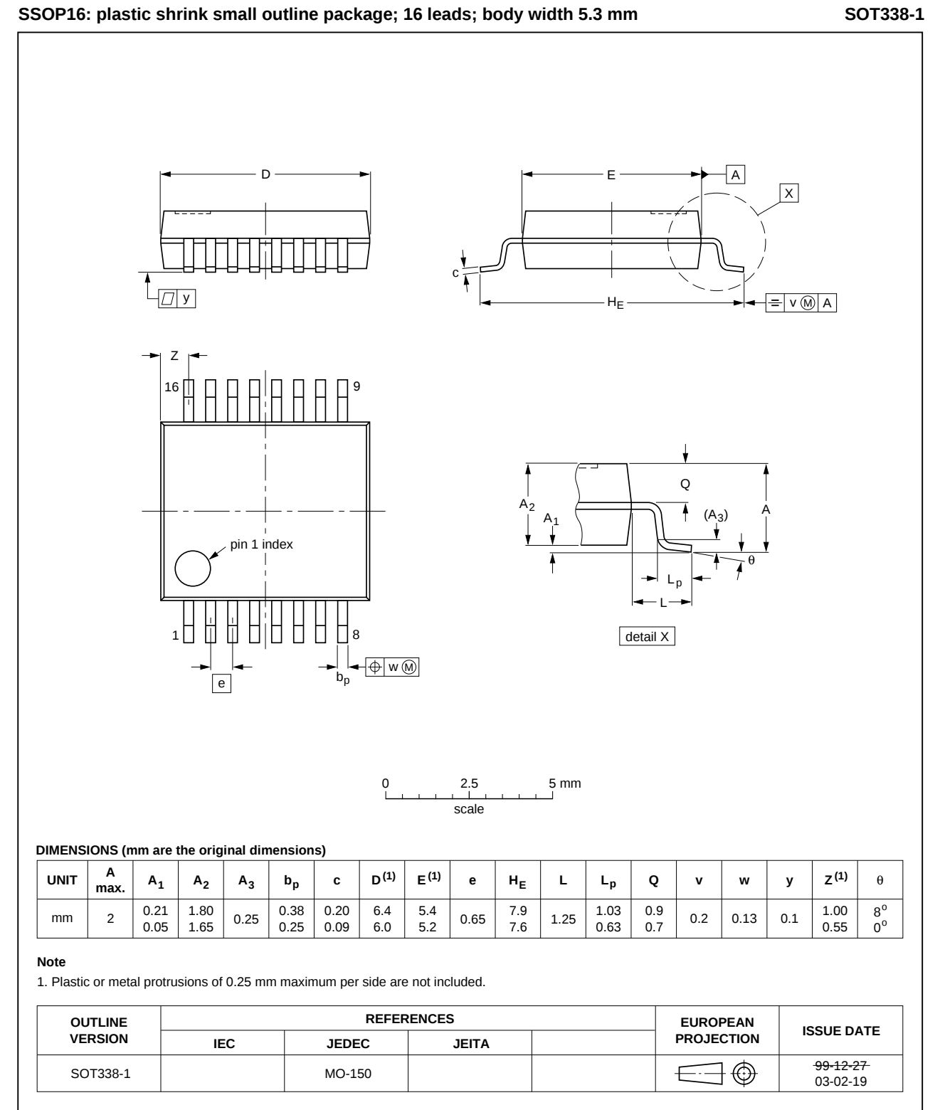
Fig 22. Package outline SOT338-1 (SSOP16)
