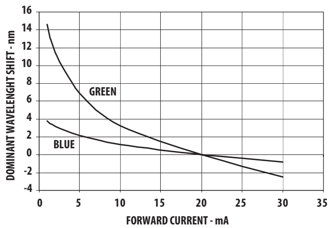
Figure 9. Relative dominant wavelength vs Forward Current
